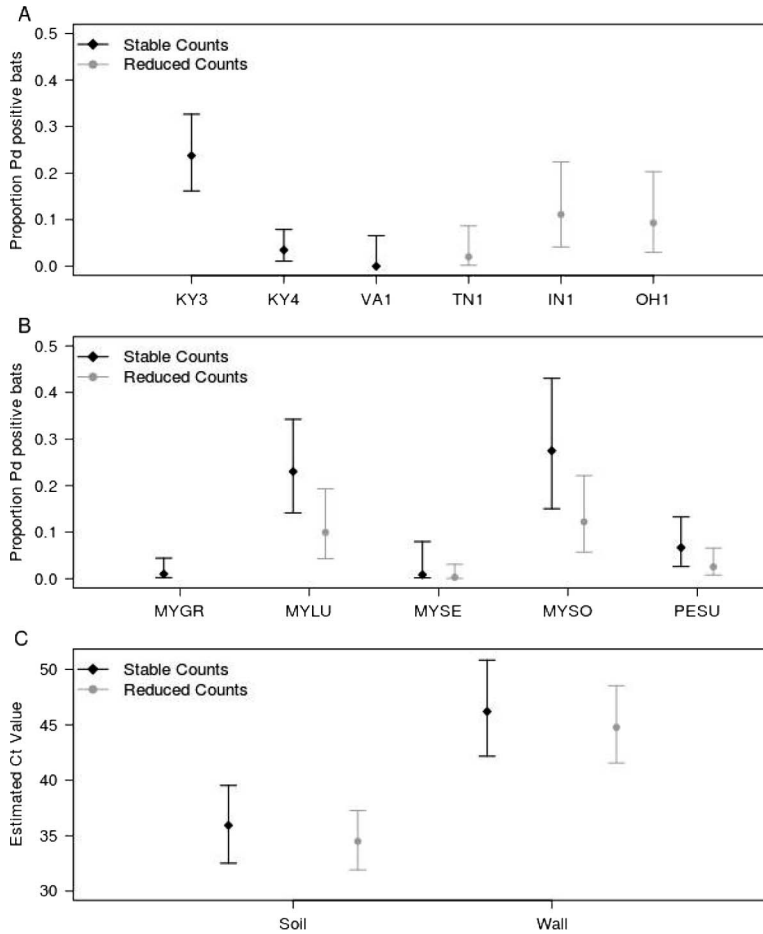
FIGURE 2. Results of PCR- and culture-based surveillance for Pseudogymnoascus destructans ( Pd ) in bats and the environment at WNS-positive hibernacula in the eastern US that were used as summer roosts between July and August, 2012. In all graphs, data-points from WNS-positive hibernacula with stable winter bat counts are black; data-points from WNS-positive hibernacula with reduced winter bat counts (>25%) are gray. Bars indicate 95% Bayesian credible intervals. a) Proportion of bats using WNS-positive hibernacula in summer that demonstrated exposure to Pd ; b) Prevalence of Pd exposure by species at WNS-positive hibernacula. (MYGR= Myotis grisescens ; MYLU= Myotis lucifugus ; MYSE= Myotis septentrionalis ; MYSO= Myotis sodalis ; PESU= Perimyotis subflavus ); c) Estimated PCR cycle threshold (Ct) values of different environmental sample types collected at WNS-positive hibernacula. “Soil” refers to floor sediment and “wall” to swabs of hibernaculum wall or ceiling substrates. Relative fungal abundance for each specimen type is inversely proportional to the Ct value.
